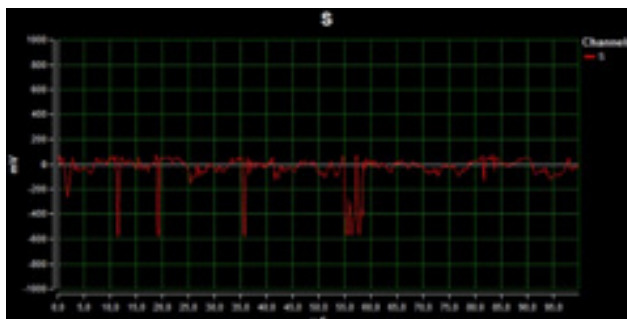
Example of sensor signal showing the signal from a small perturbation of the cable.
