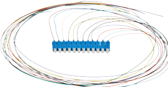
SL Pigtail 0,9mm SM G657 SCUPC S12, 1.5m, 12pcs/package
