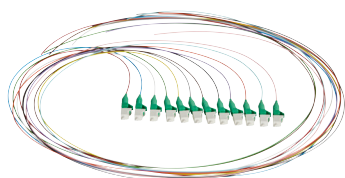
SL Pigtail 0,9mm SM G657 LCAPC S12, 1.5m, 12pcs/package
