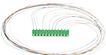
SL Pigtail 0,9mm SM G657 SCAPC S12, 1.5m, 12pcs/package
